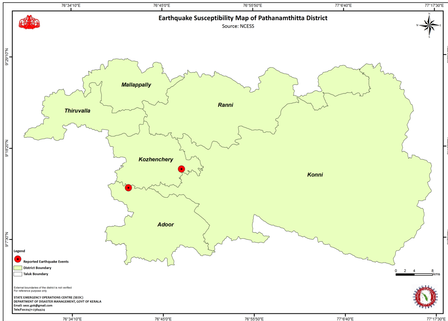
FIGURE 11: EARTHQUAKE SUSCEPTIBILITY MAP OF PATHANAMTHITTA DISTRICT (ANNEXURE 32)
