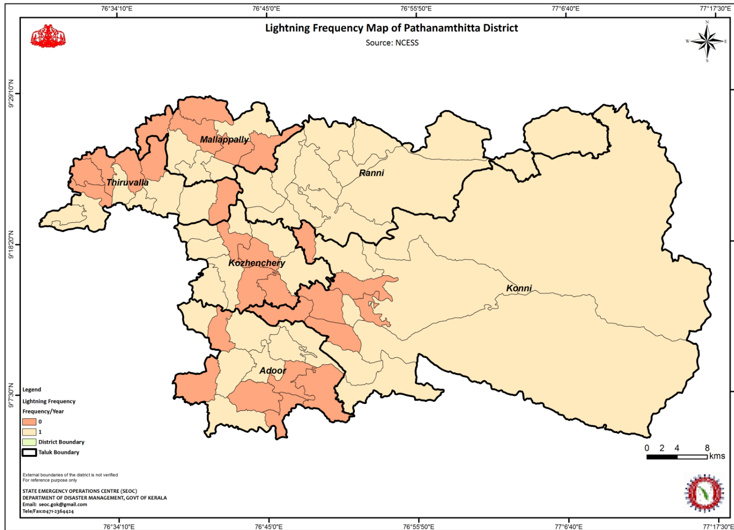
FIGURE 13: LIGHTNING FREQUENCY MAP OF PATHANAMTHITTA DISTRICT (ANNEXURE 34)
