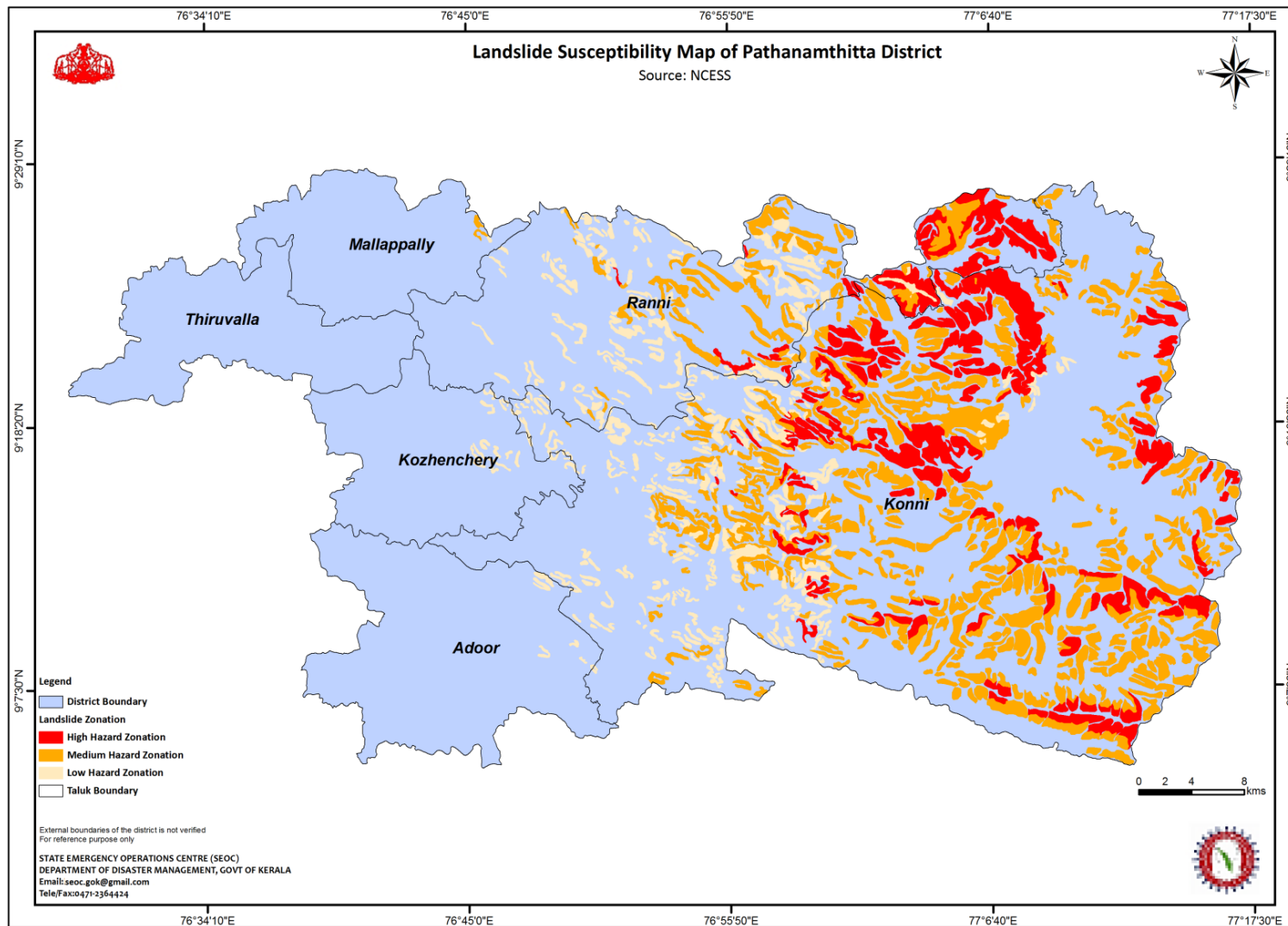
FIGURE 12: LANDSLIDE SUSCEPTIBILITY MAP OF PATHANAMTHITTA DISTRICT (ANNEXURE 30)
