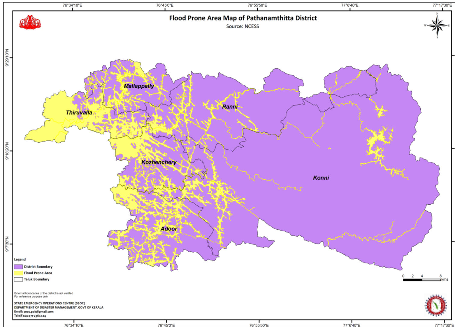
FIGURE 9: FLOOD PRONE AREA MAP OF PATHANAMTHITTA DISTRICT (ANNEXURE 30)
